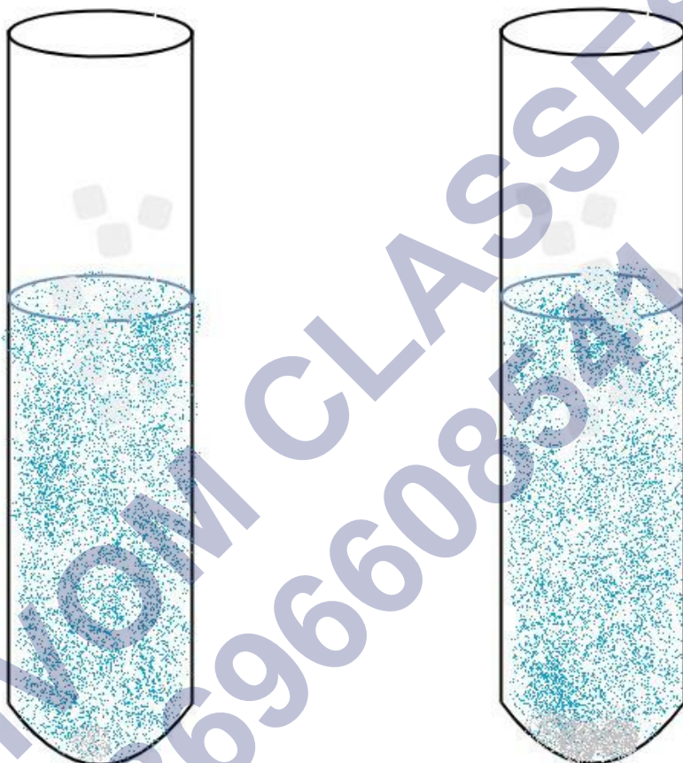
Unsaturated Solution
