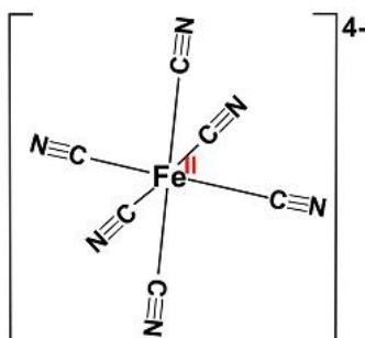
Octahedral Geometry
